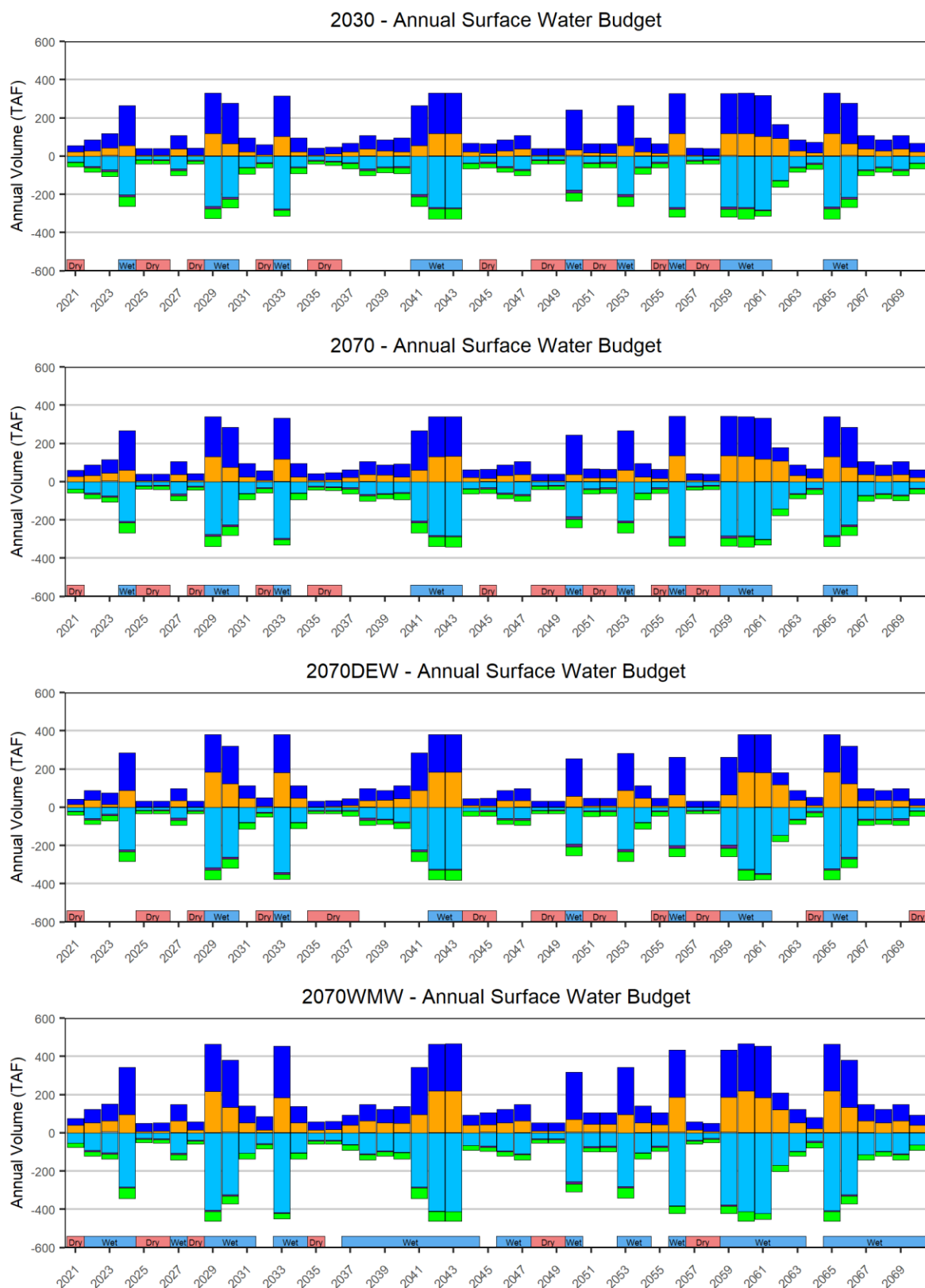
Figure 2.2.3-15. Projected future surface water budgets.
