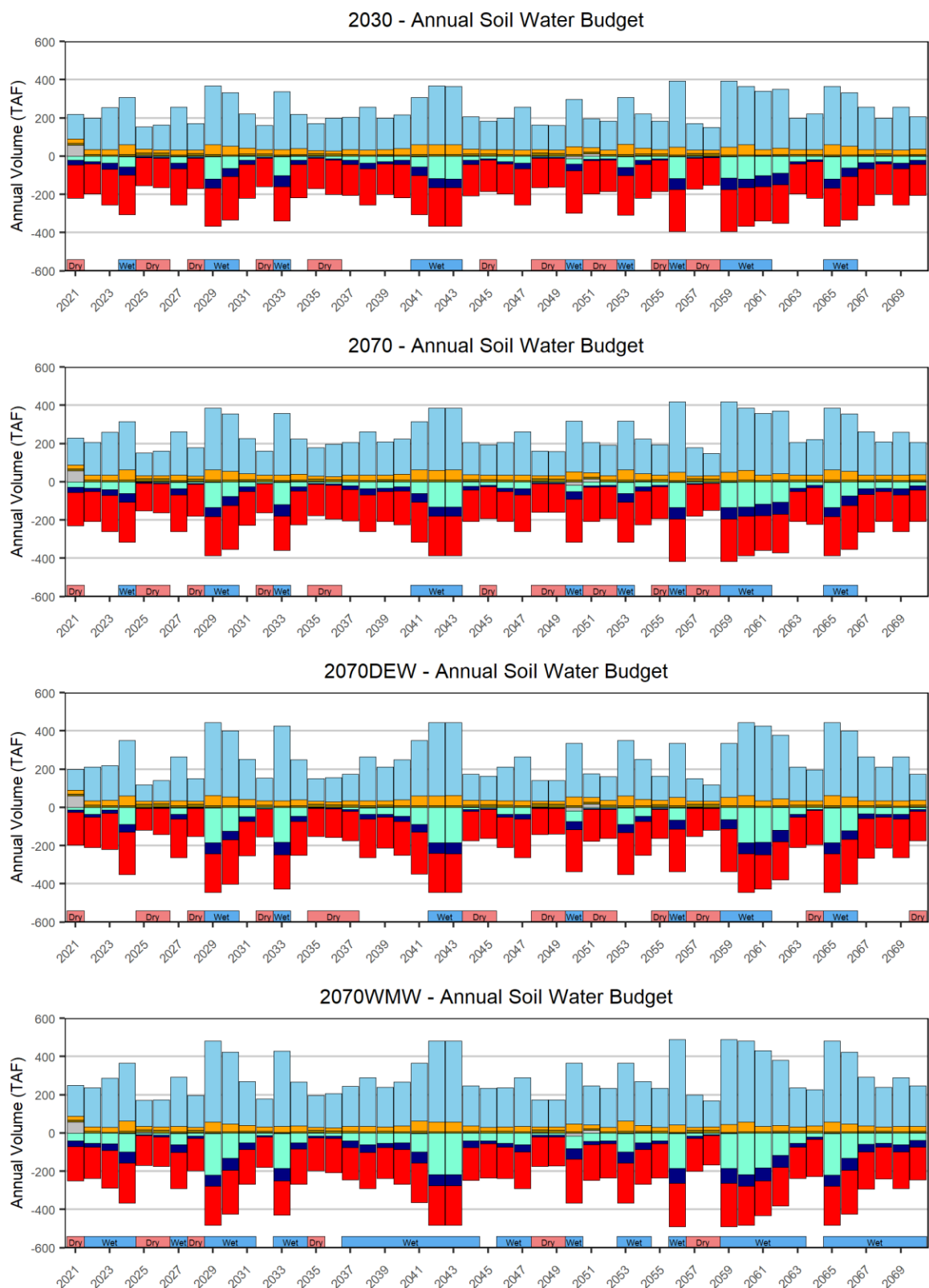
Figure 2.2.3-16. Projected groundwater basin future land surface water budgets.
