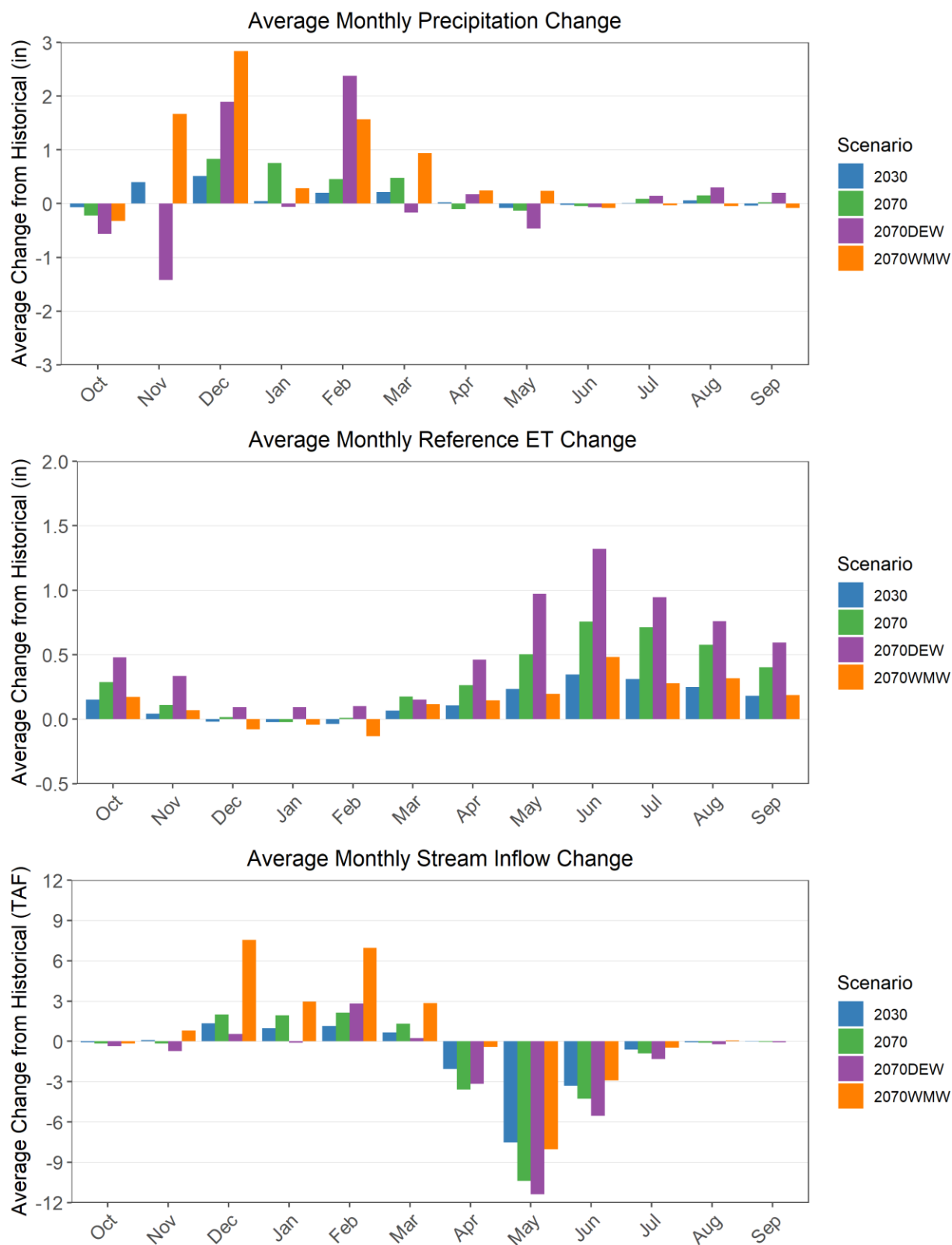
Figure 2.2.3-11. Average change from historical inputs by month using DWR climate change factors.
