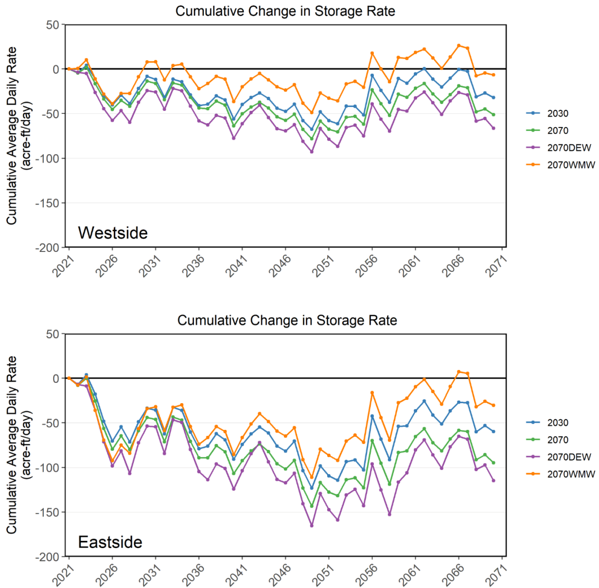
Figure 2.2.3-19. Eastside portion of the basin projected to experience greater declines in groundwater storage than the westside in the future.
