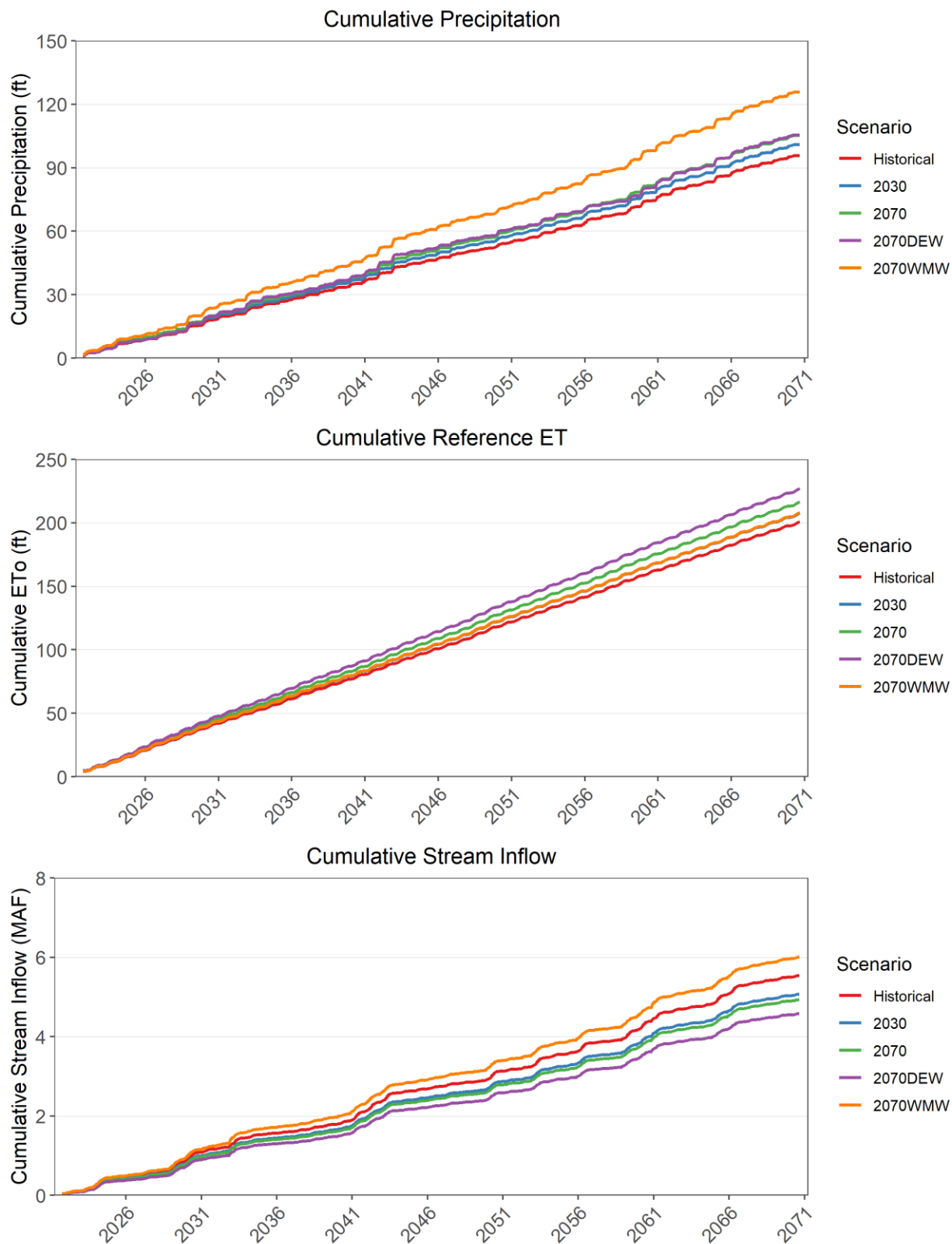
Figure 2.2.3-10. Cumulative inputs of future climate using DWR climate change factors.
