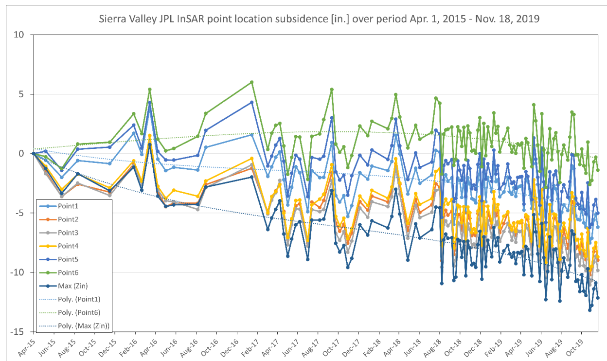
Figure 2-32 Time series of JPL InSAR land subsidence data for the locations called out in Figure 2.2.2-3
