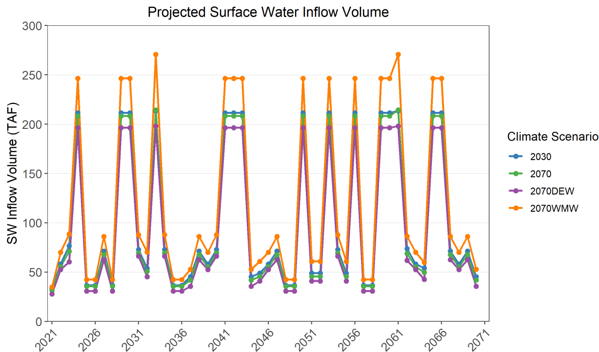
Figure 2.2.3-14. Projected surface water inflow to Sierra Valley.
