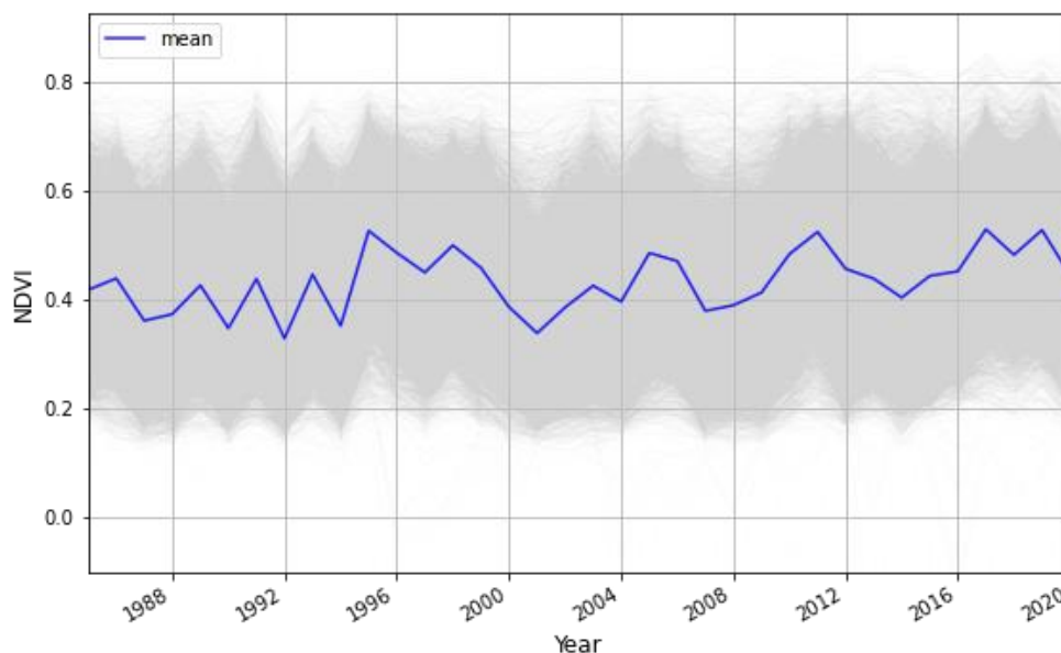
Figure 2-39 Summer NDVI changes through time in the Sierra Valley Subbasin. The blue line is the mean value of the GDE polygons
