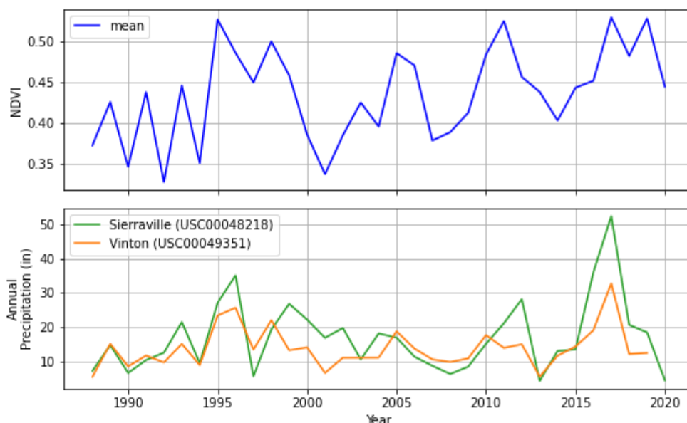
2506 Figure 2-40 Mean summer NDVI and annual precipitation at Sierraville and Vinton
