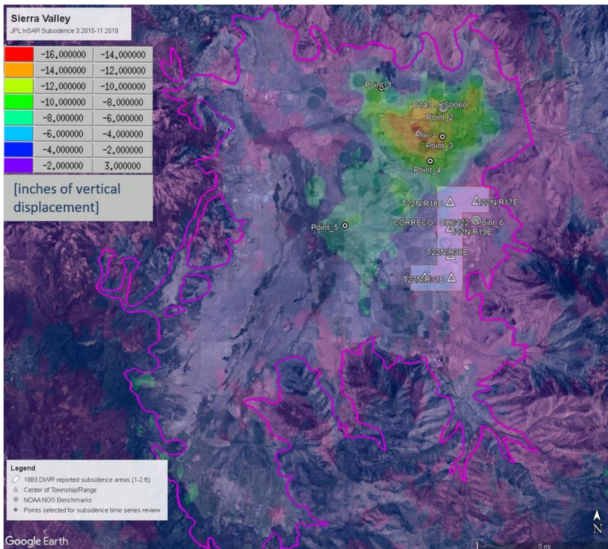
2015 Figure 2-30 InSar-based land subsidence for the period of March 2015 to November 2019
