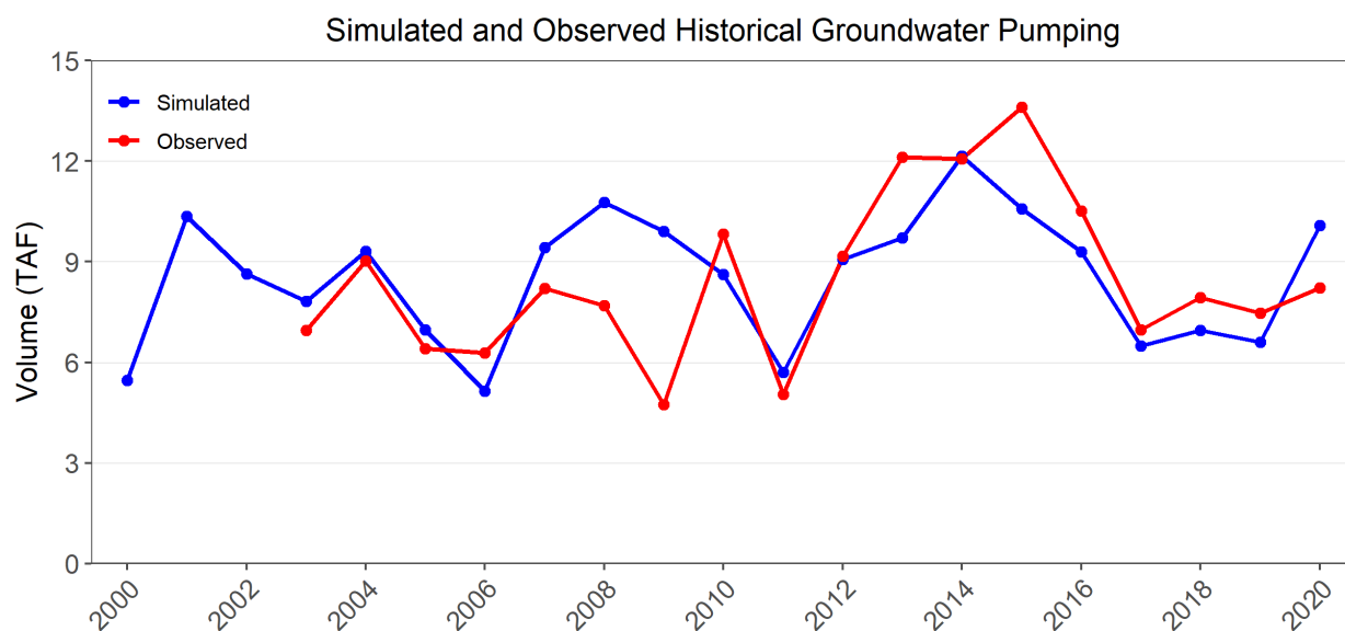
Figure 2.2.3-12. Historical groundwater pumping is well represented for most years by SVHSM.
