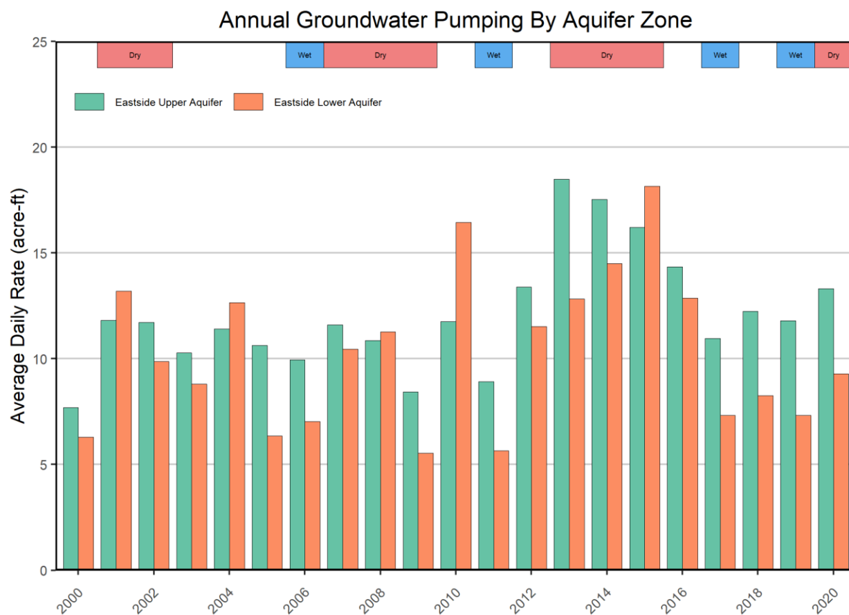
Figure 2.2.3-9 Historical and Current Annual Pumping Rates by Aquifer Zone
