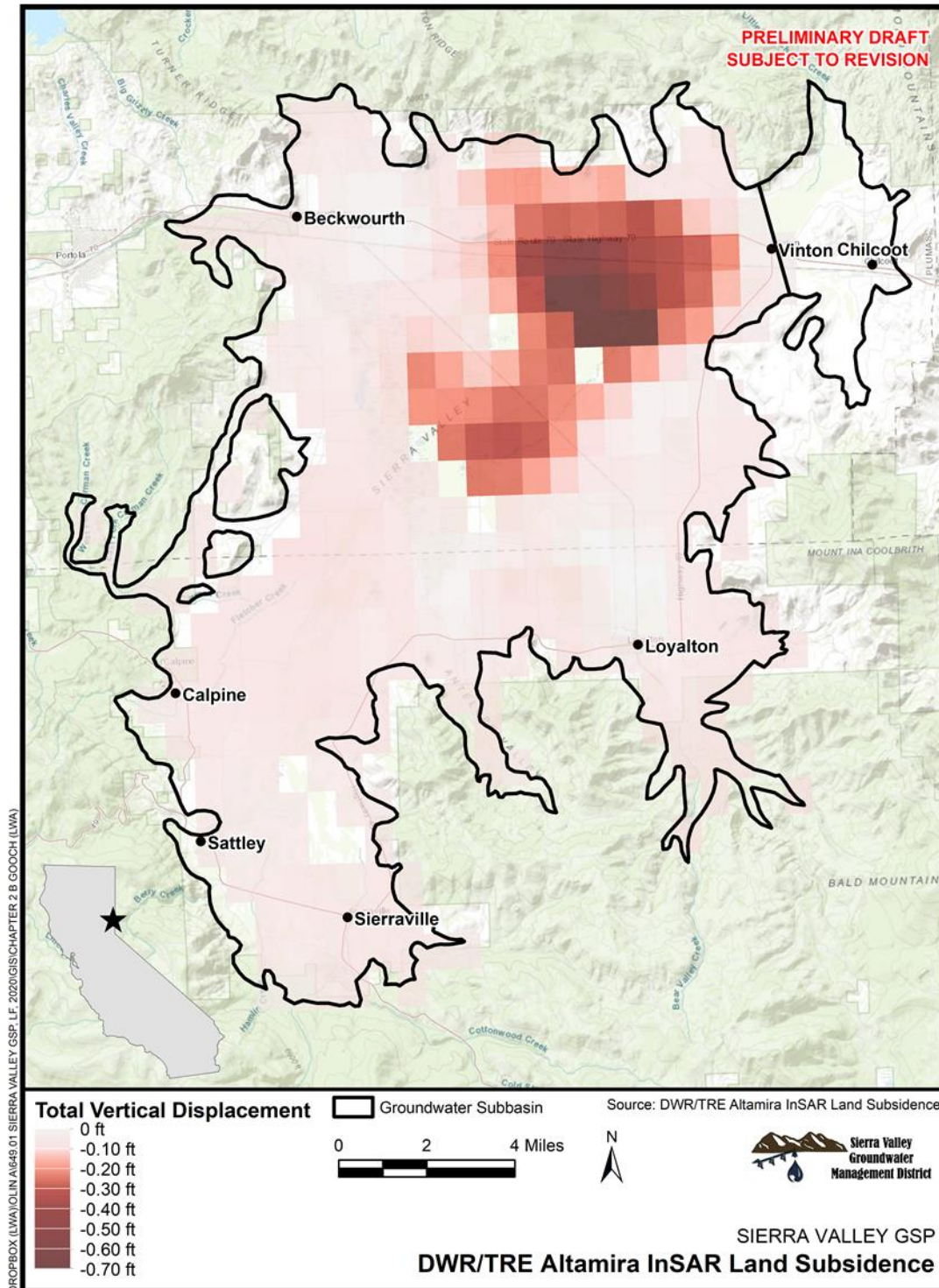
Figure 2-33 DWR/TRE Altamira InSAR land subsidence for the period June 2015 to September 2019
