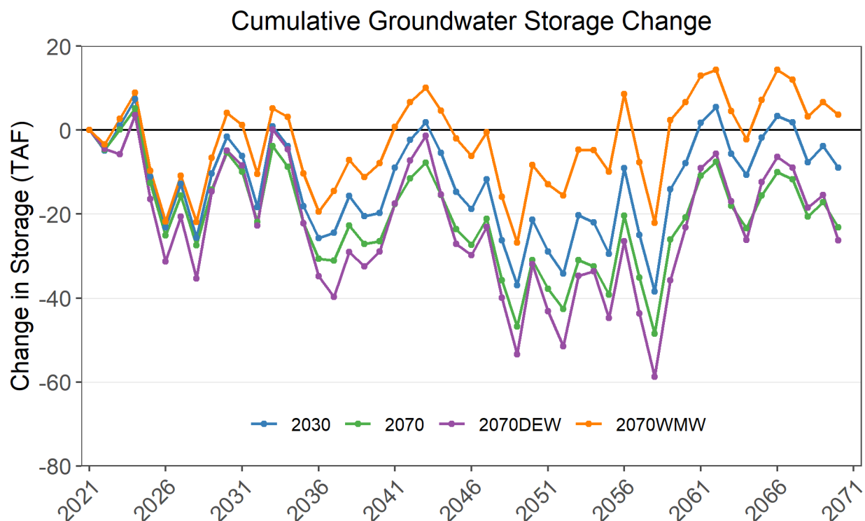
Figure 2.2.3-18. Projected change in groundwater storage from climate change scenarios.
