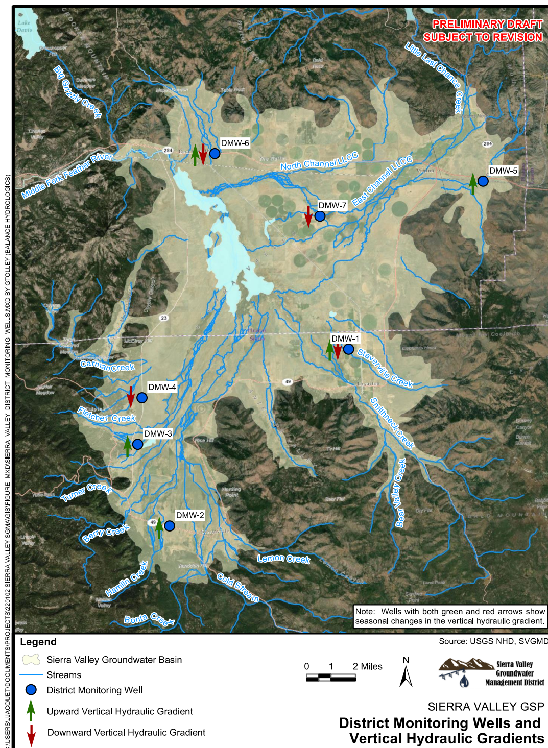
Figure 2-35 Locations of district monitoring wells in the Sierra Valley. Wells with both green and red arrows show seasonal changes in the vertical hydraulic gradient
