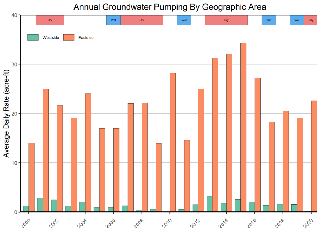
Figure 2.2.3-7 Historical and Current Annual Pumping Rates by Geographic Area
