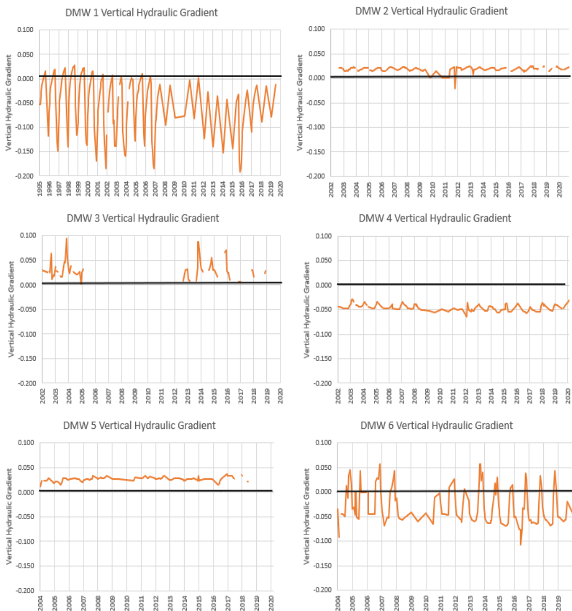
Figure 2-34 Calculated vertical hydraulic gradients between deep and shallow nested district monitoring wells
