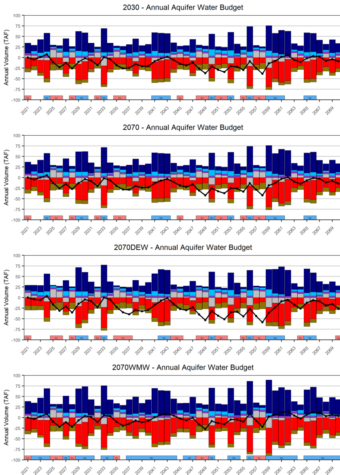
Figure 2.2.3-17. Projected future groundwater budgets.
