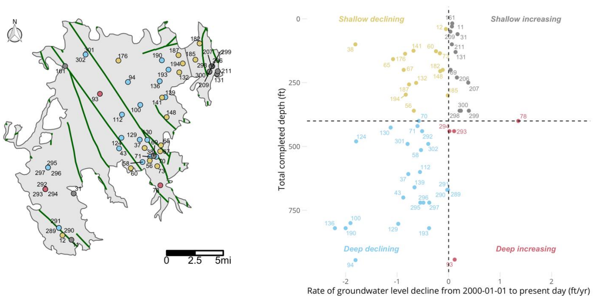
1542 1543 Figure 2-26 Sierra Valley Groundwater Level Trends for Deep and Shallow Wells
