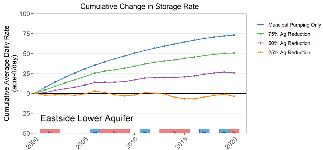
Figure 2.2.3-22. SVHSM predicts a 25-35% reduction in agricultural groundwater pumping would arrest declining storage in the eastside lower aquifer.
