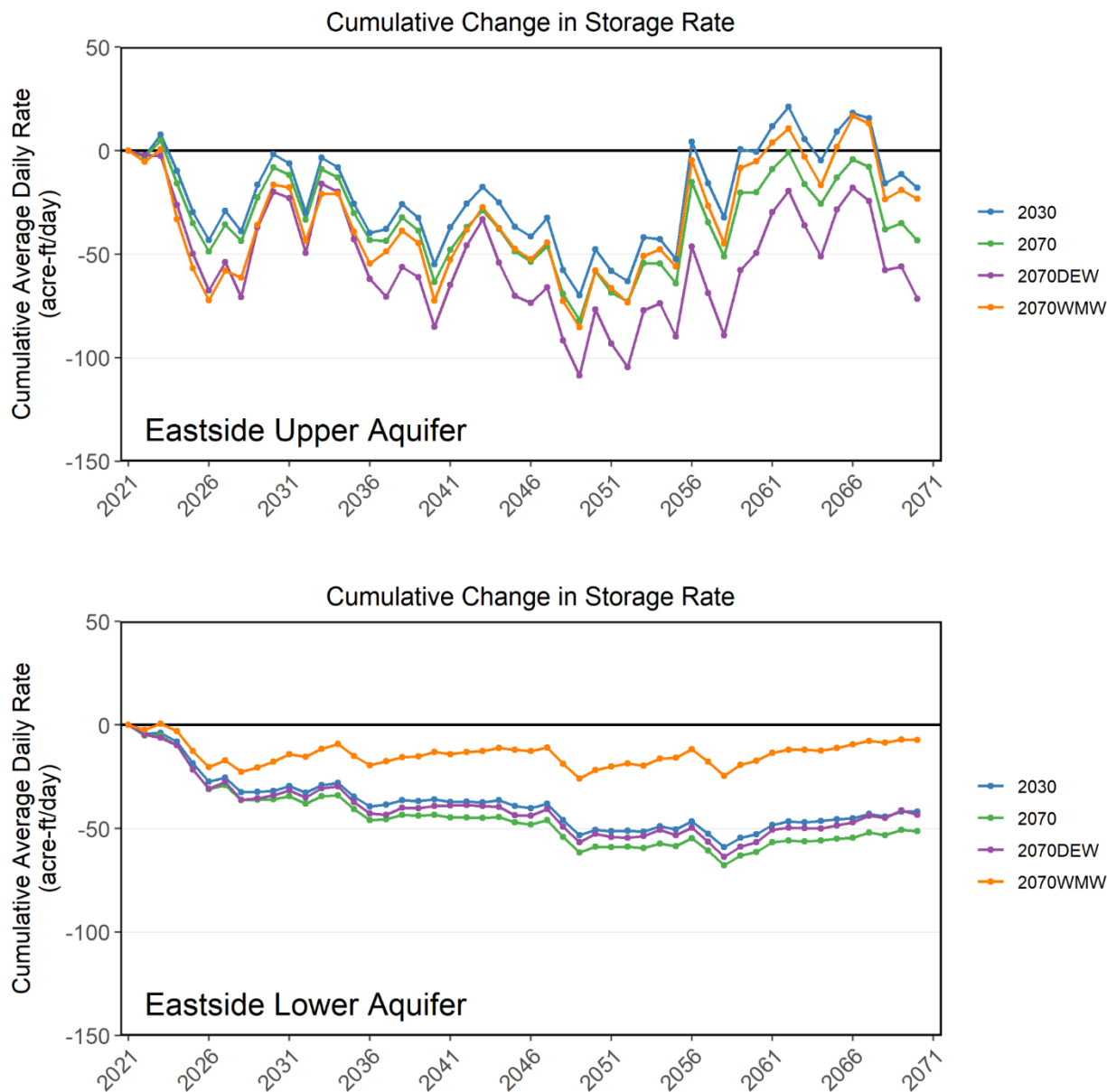
Figure 2.2.3-20. Continued declines in groundwater storage are expected for the eastside lower aquifer in the absence of management changes.
