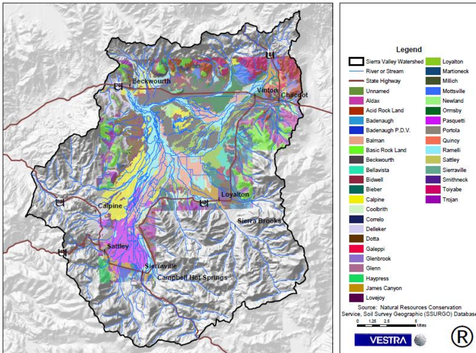
Figure 2.2-2. Sierra Valley Soils (Vestra, 2005).
