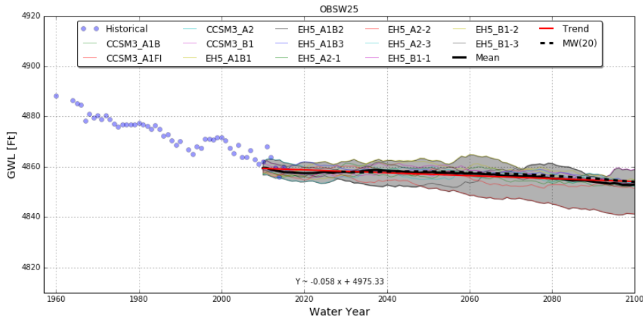
Figure 2.2-33. Long-term Hydrograph Projections for Loyalton Area (Dib et al., 2017).
