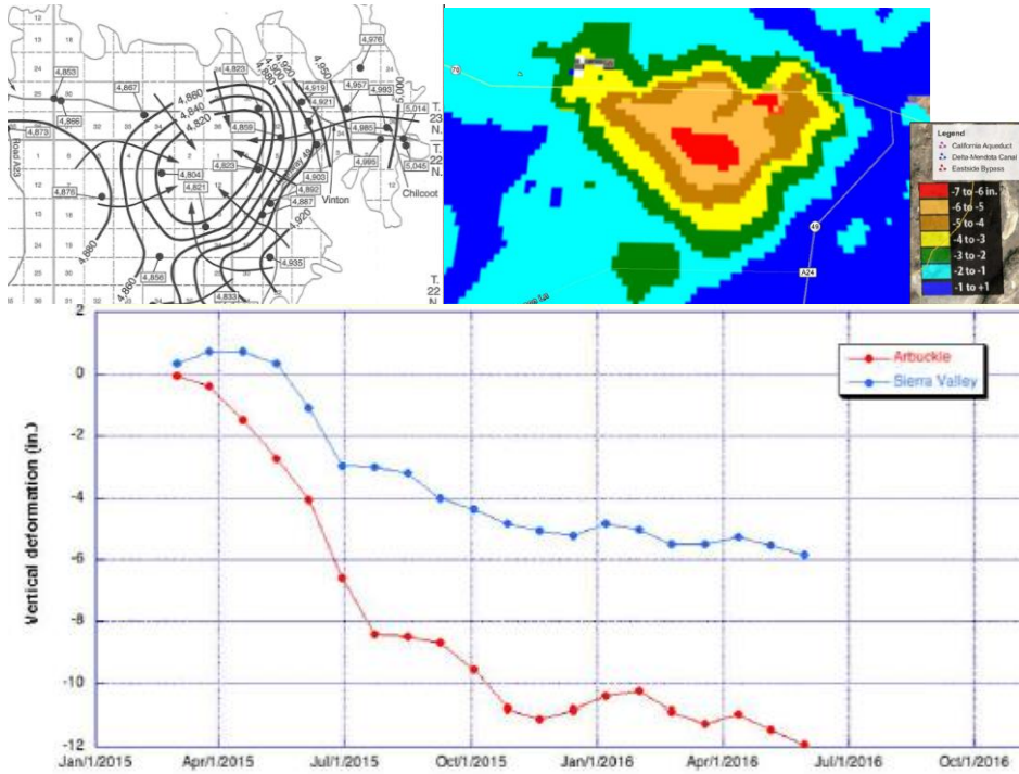
Figure 2.2-35. Maps and Graph showing InSAR land subsidence data (Farr et al., 2017) with location/extents consistent with groundwater level contours for the same time period (Schmidt, 2017).
